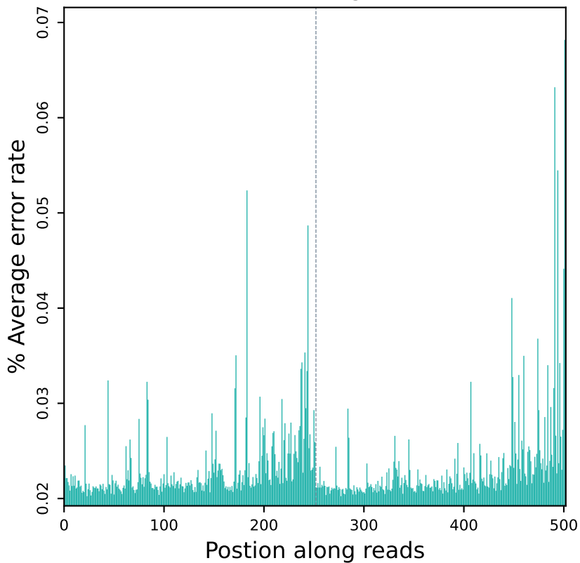
Error rate distribution along reads (R20218)
